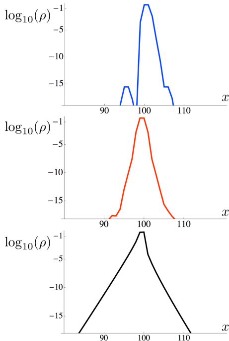
FIG. 2. (Color online) Logarithmic plots of the probability density \rho of WFs with home cell x = 101 for a non-trivial 1D TSC with \mu = 0.3, 2t = 2\Delta = 1 (see Section II C for definitions). Upper panel: Result of algorithm without additional symmetries and coupling constants \xi = 10, r = 50, \lambda = 20 . Central panel: Result of algorithm with \mathcal{S} = \{\text{PHS}\} and coupling constants \xi = 10, r = 50, \lambda = 20 . Lower panel: WF from the gauge constructed in Eq. (20). L = 200 has been chosen for all plots.
