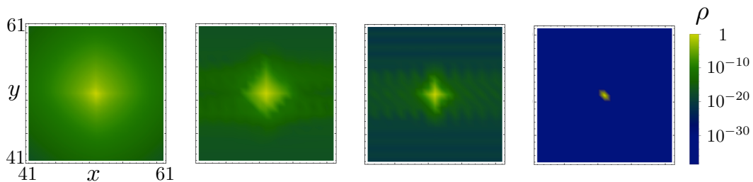
FIG. 4. (Color online) Logarithmic plot of the probability density \rho of an initial Wannier function for the model Hamiltonian (22) for the topologically trivial mass parameter M = 2.5 (leftmost panel). The home cell of the WFs is (x, y) = (51, 51) , the size of the lattice is 101 \times 101 . Adiabatically deformed WF after 100, 500, and 727 iterations respectively with \xi = \kappa = \lambda = 50 .
